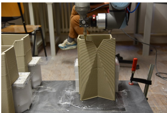
Figure 35: Documentation of 3D printing of the climate performative tile
