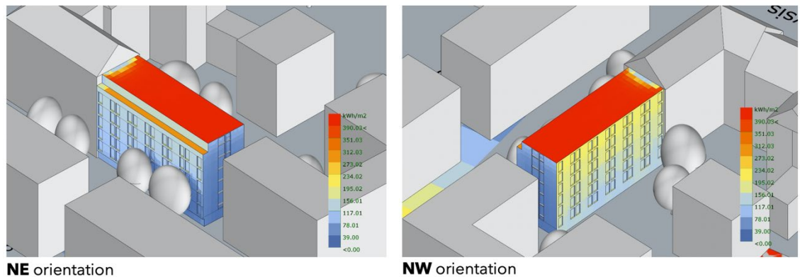
Figure 17: Solar radiation analysis
