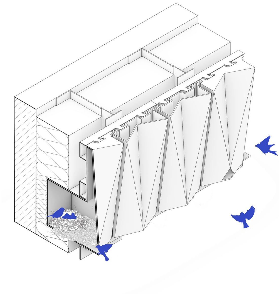
Figure 25: Axonometry section of the façade fragment
