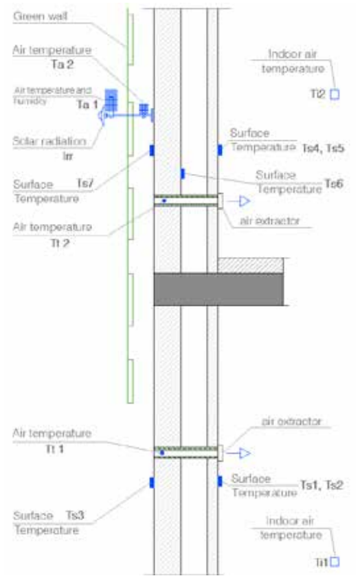
FIG. 3 Monitoring system
