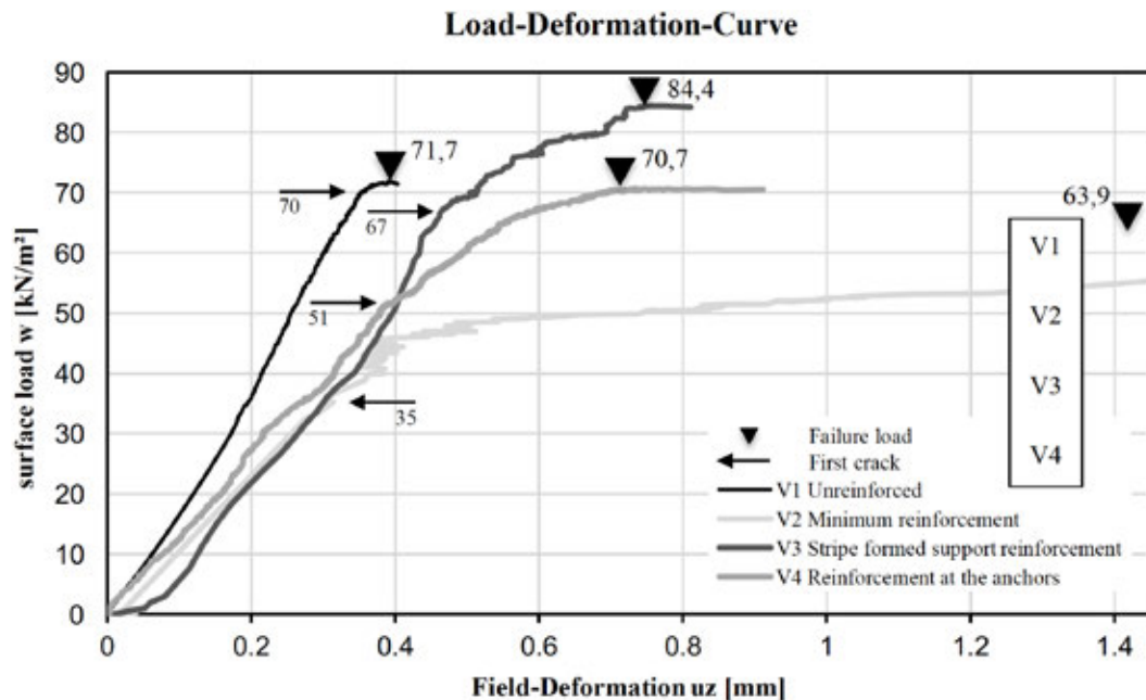
FIG. 6 Load-deformation-diagram
