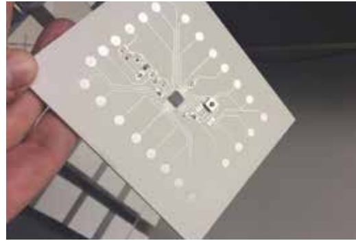
FIG. 6 Prototype of a PACE ultra thin textile reinforced concrete element with a freely programmable control unit for Agile Compounds R&D: BAU KUNST ERFindEN // BUILDING ART INVENTION, University of Kassel, J. Iwanowicz, T. Klooster and H. Klussmann, Photo: BAU KUNST ERFindEN
