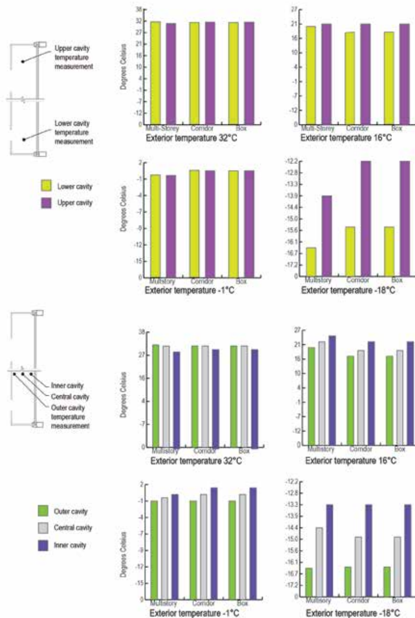
FIG. 2 Results of heat transfer analysis, showing temperatures in air cavity for investigated DSFs
