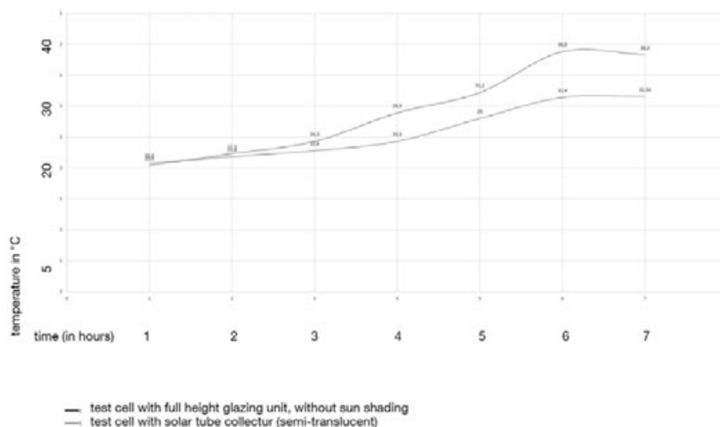
FIG. 5 thermal behavior of two test cells on a summer day. (21.07.2010)
