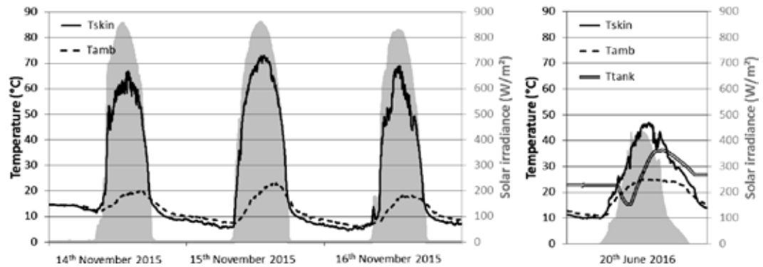
FIG. 7 Temperatures of ambient air (Tamb), skin (Tskin) and tank (Ttank) and solar irradiance (gray shaded area) for selected days measured during experimental test of (BASSE, 2016) at KUBIK test facility
