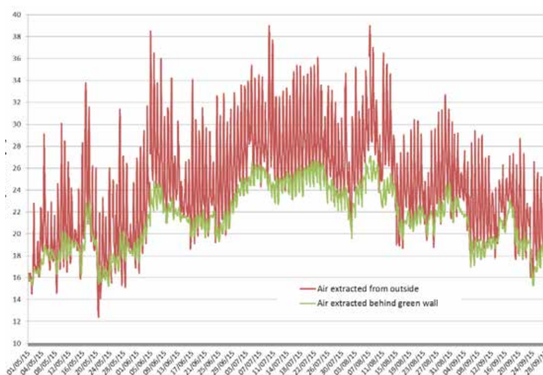
FIG. 7 Comparison between the temperatures of the outside extracted air in presence or in absence of the vertical greening system during summer period
