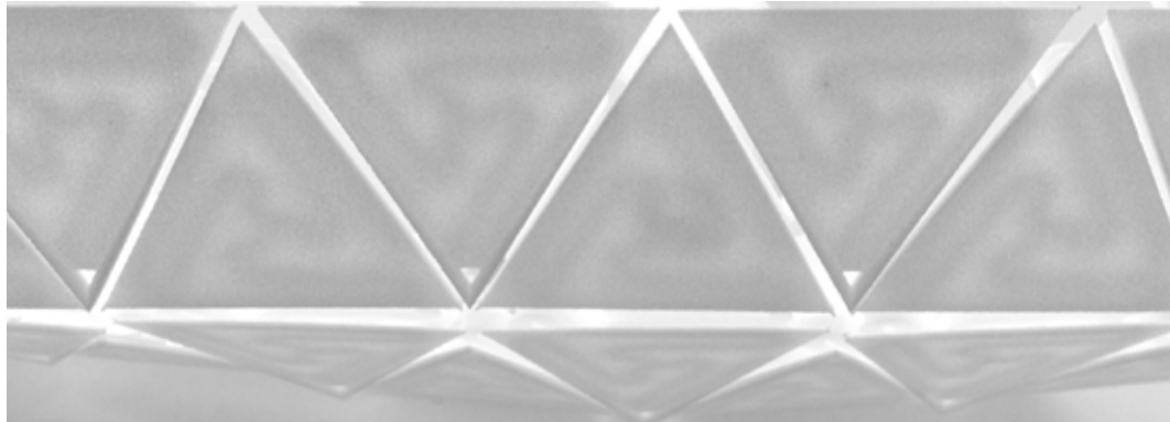
FIG. 9 3d-printed model of an auxetic geometry with weather protection discs and movable ventilation gaps
