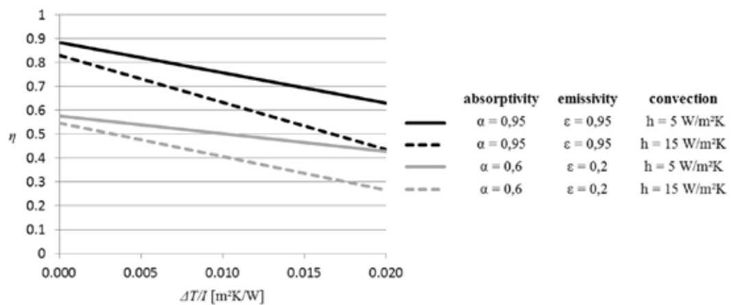
FIG. 9 Simulated performance of BATISOL solution as a function of temperature differential divided by solar irradiance (Bonnamy, Raji, Lopez, & Garay, 2016). The four scenarios combine an external surface of galvanised steel ( \alpha = 0,6 ; \epsilon = 0,2 ) or matt black coating ( \alpha = 0,95 ; \epsilon = 0,95 ) with low ( h = 5 \text{ W/m}^2\text{K} ) or moderate ( h = 15 \text{ W/m}^2\text{K} ) wind conditions
